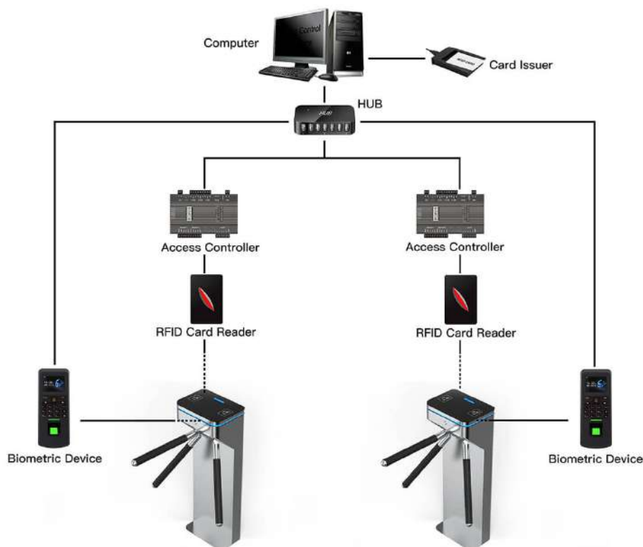
Nebula Tripod Turnstile DSN-50
